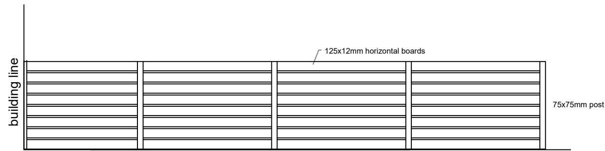
existing fence elevation scale 1:50
